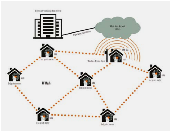
Figure 1: CyanConnode RF Mesh Configuration
