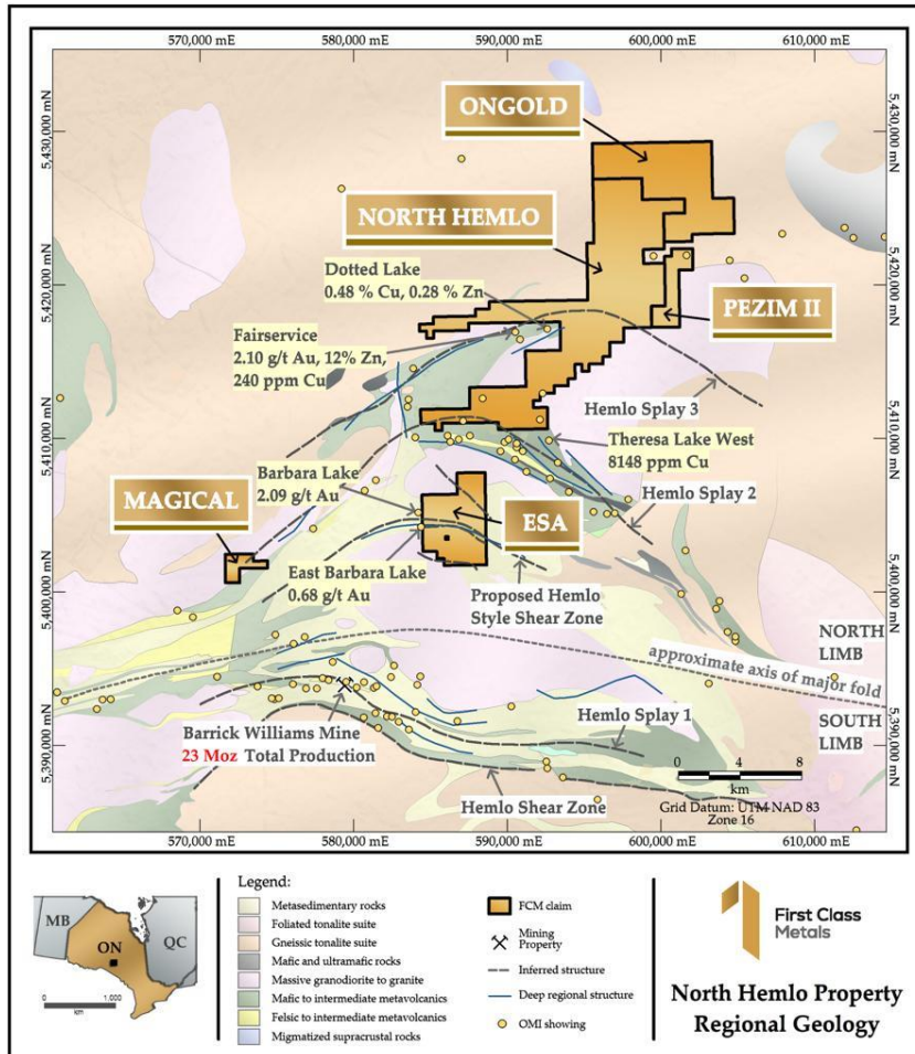
Figure showing the relative location of North Hemlo (including OnGold), Esa and Magical in respect to the Williams gold mine and the district scale shears associated with mineralisation
